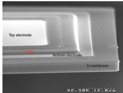
▲ SEM image of the free end of a MEMS micro-cantilever beam integrating a KNN layer
