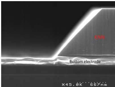
▲ SEM photograph of a thin KNN layer after etching
